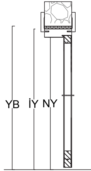
Dikey Kesit Vertical Cross Section
