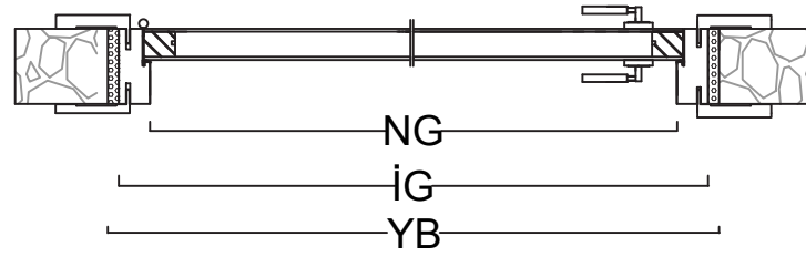
Yatay Kesit Horizontal Cross Section
